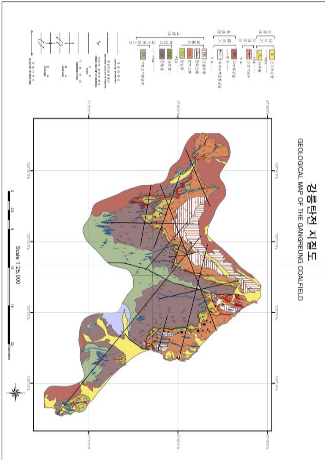
Figure 1. Digital coal geological map of Gangneung coal field
