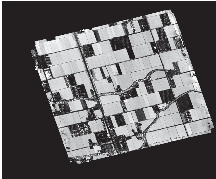
Supplementary Fig. 3. Difference DEM on September 28, 2021. DEM, digital elevation model.
